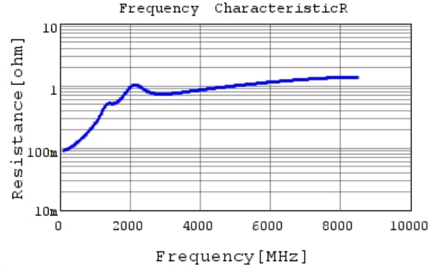
GRM1552C1H221JA01 R DCOV, 20degC
