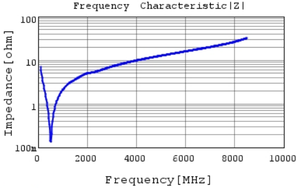
GRM1552C1H221JA01 |Z| DCOV, 20degC
