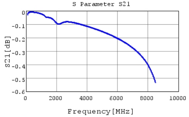
GRM1552C1H221JA01 S21 DCOV, 20degC
