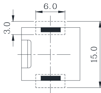
Recommendable Land Pattern
