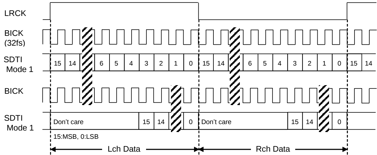
Figure 34. Mode 1 Timing
