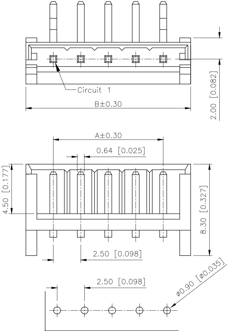
PCB LAYOUT
