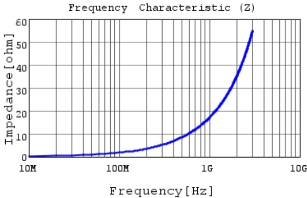
LQP03TN2N7C02 |Z|
