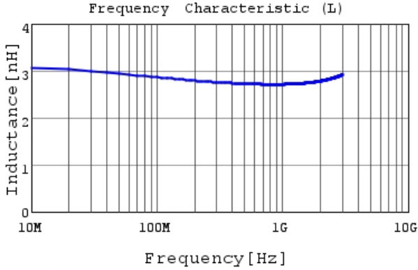
LQP03TN2N7C02 L
