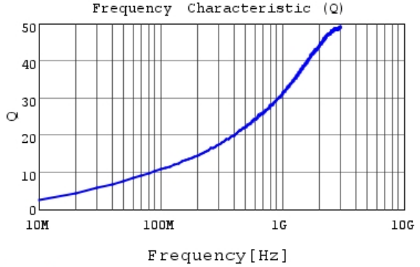
LQP03TN2N7C02 Q
