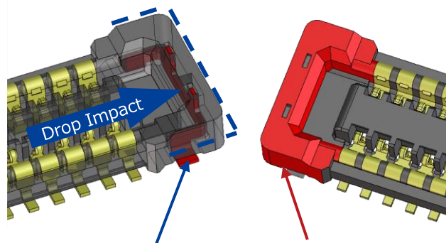
Metal solder tabs absorb the stress by drop impact
