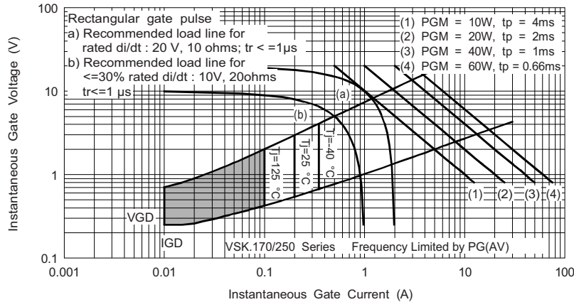
Fig. 23 - Gate Characteristics
