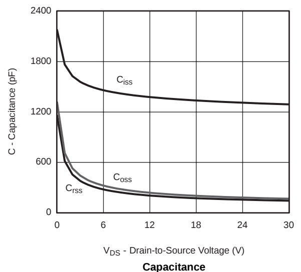
Capacitance
