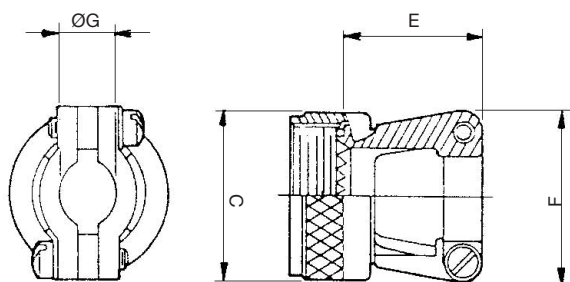
Wire Bundle Accommodation without resilient bushing
