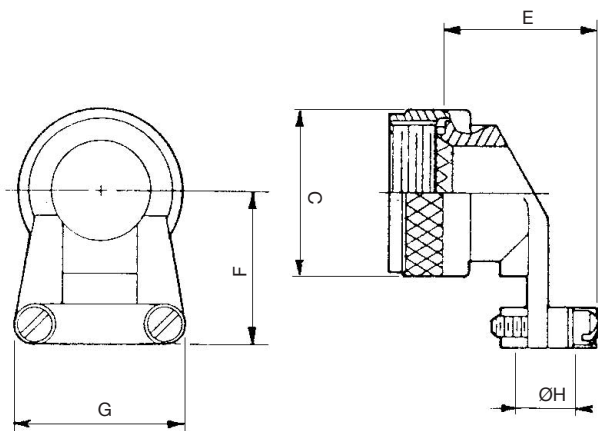
Wire Bundle Accommodation without resilient bushing
