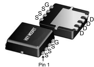
DFN3X3-8L (TSDSON-8-EP(3.3x3.3))
