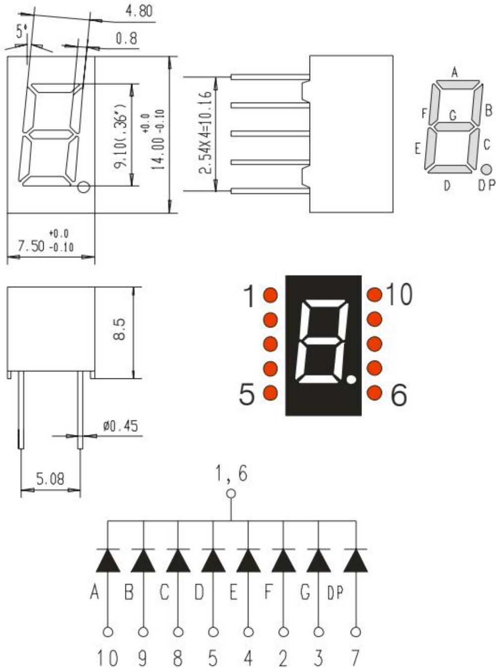
Figure Size & Circuit Principle Diagram : 7.5mm×14mm×8.5mm
