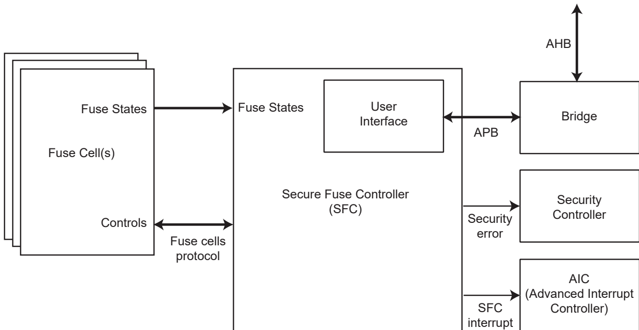
Figure 56-1. SFC Block Diagram
