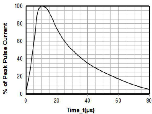
8 X 20 \mu\text{s} Pulse Waveform
