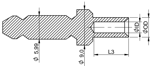
sectional drawing A-A
