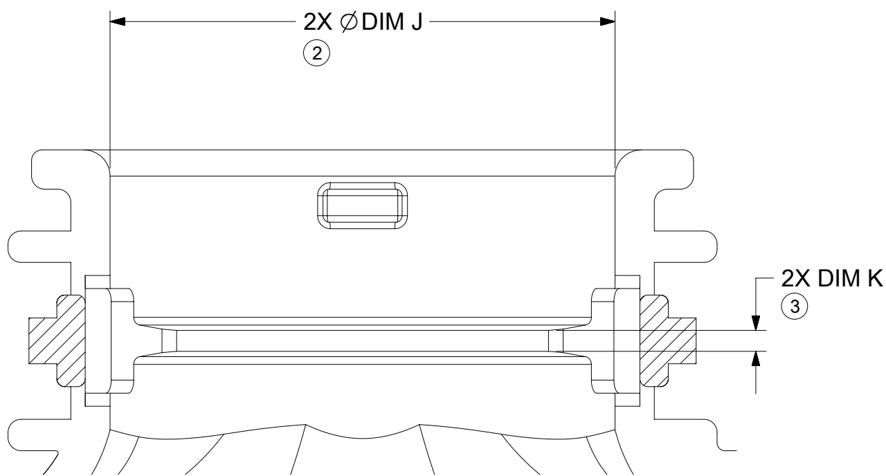
PARTIAL SECTION C-C SCALE 5:1 WITH RIBS
