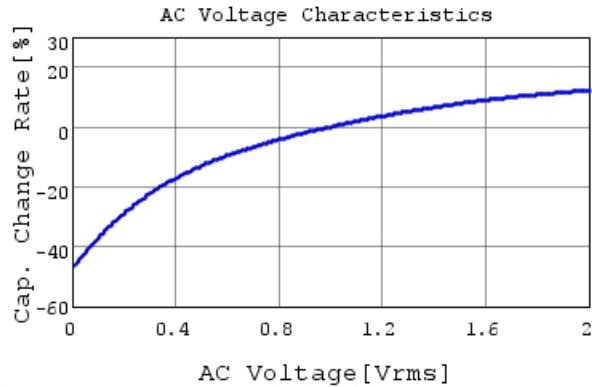
GRM155R61C474KE01 C-AC Voltage capchange, DC
