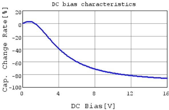
GRM155R61C474KE01 C-DC bias capchange, 25.0c
