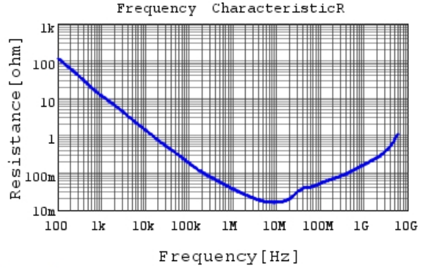
GRM155R61C474KE01 R DCOV, 25degC
