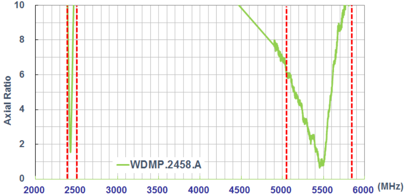
Figure 6. Axial Ratio
