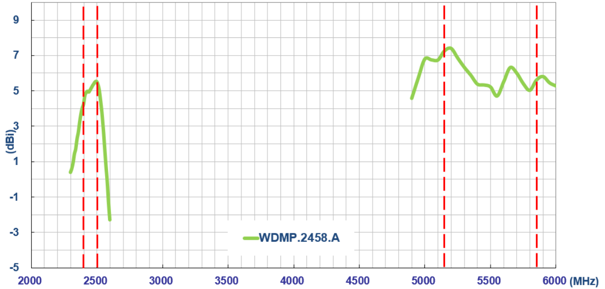
Figure 4. Peak Gain.
