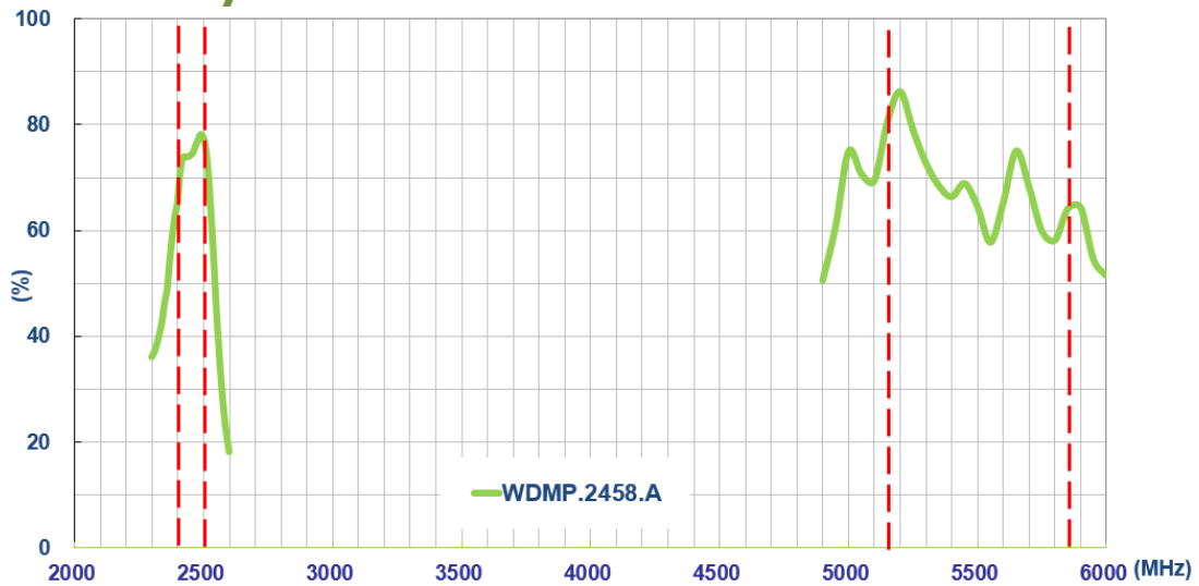
Figure 3. Efficiency
