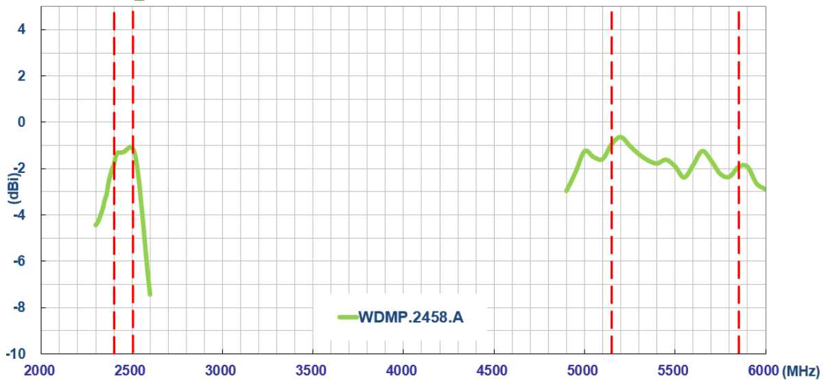
Figure 5. Average Gain
