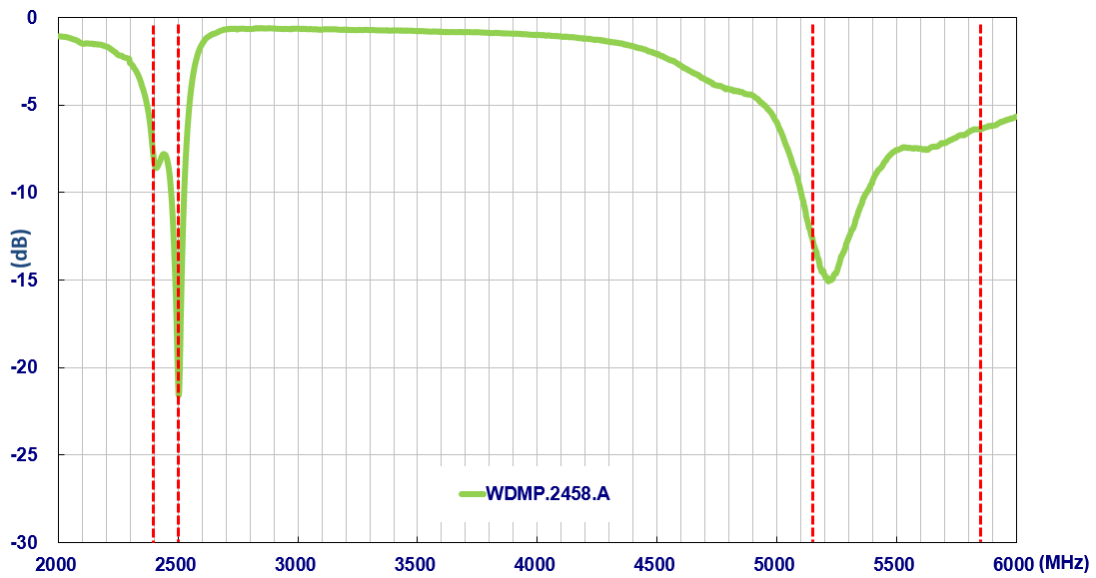
Figure 2. Return Loss
