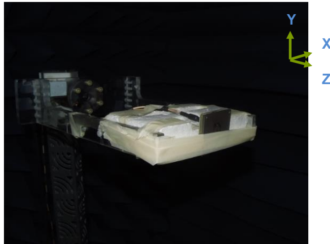
Figure 1. Peak gain, efficiency and radiation pattern measurements
