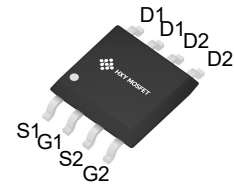
SOP-8 (SO-8-150mil)
