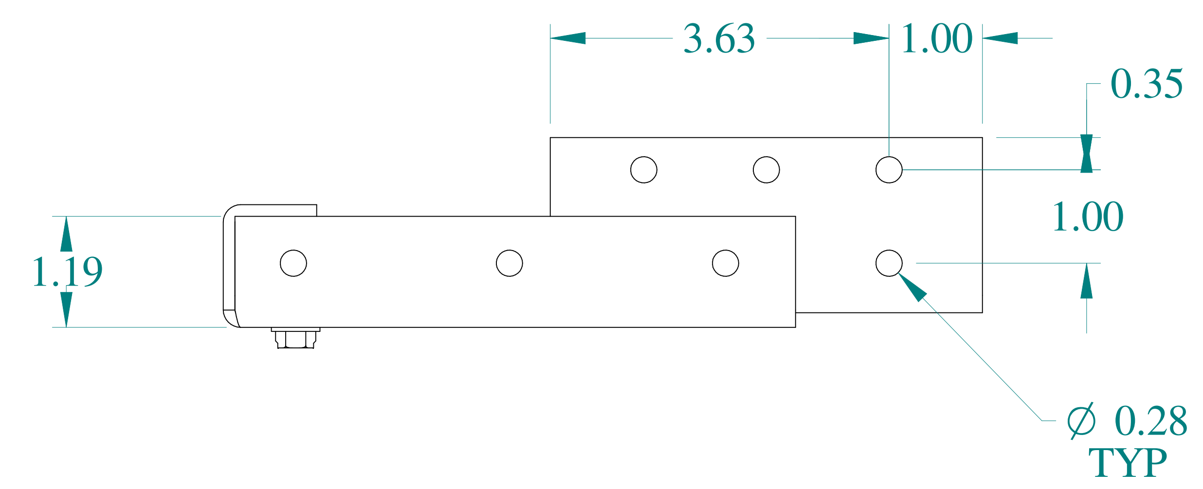
TOP VIEW
