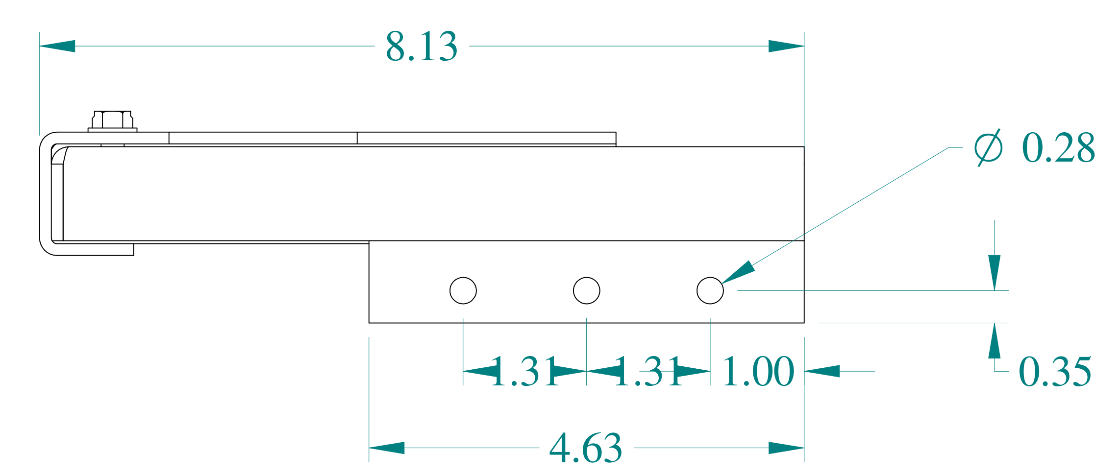
BOTTOM VIEW
