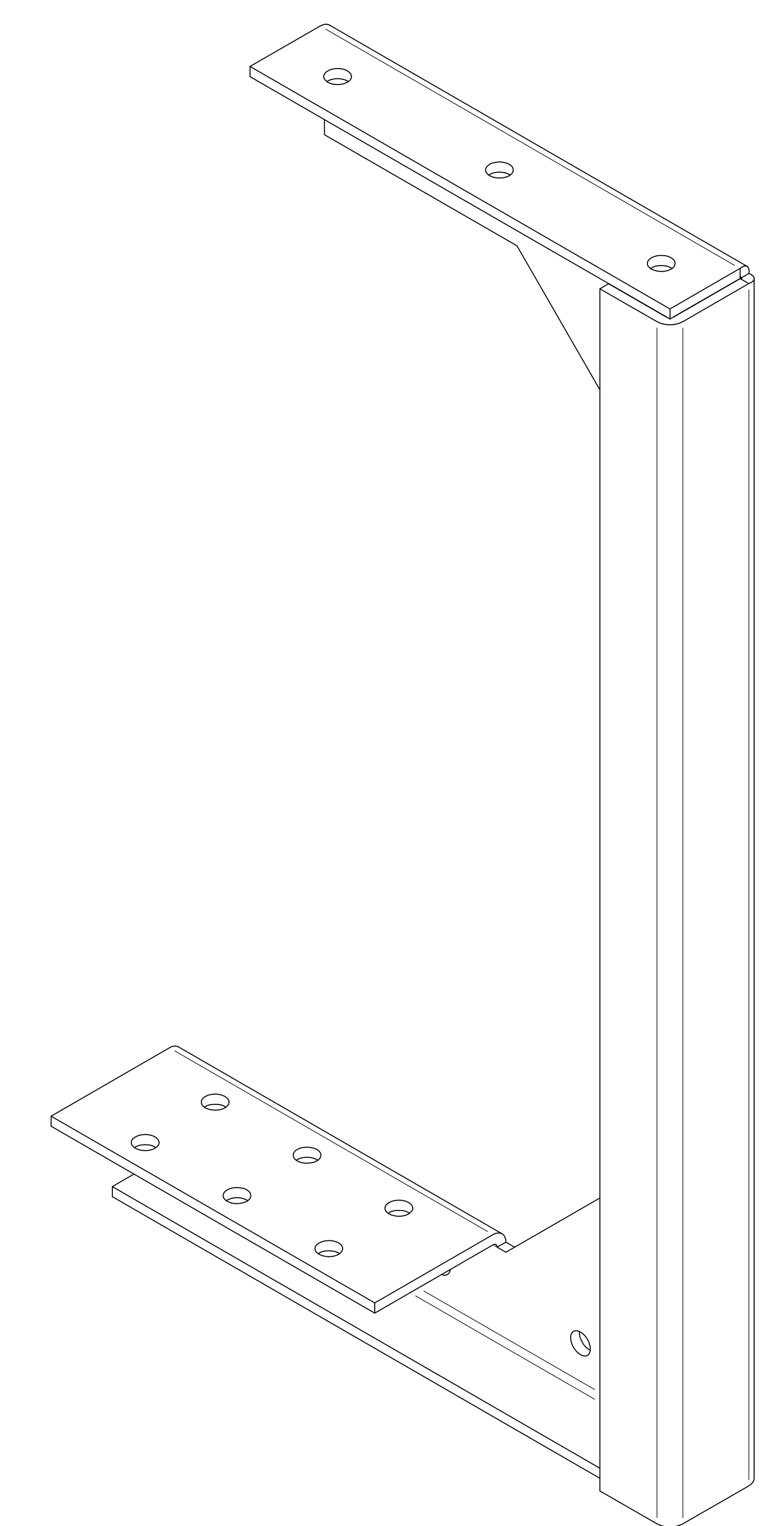
ISOMETRIC VIEWS
