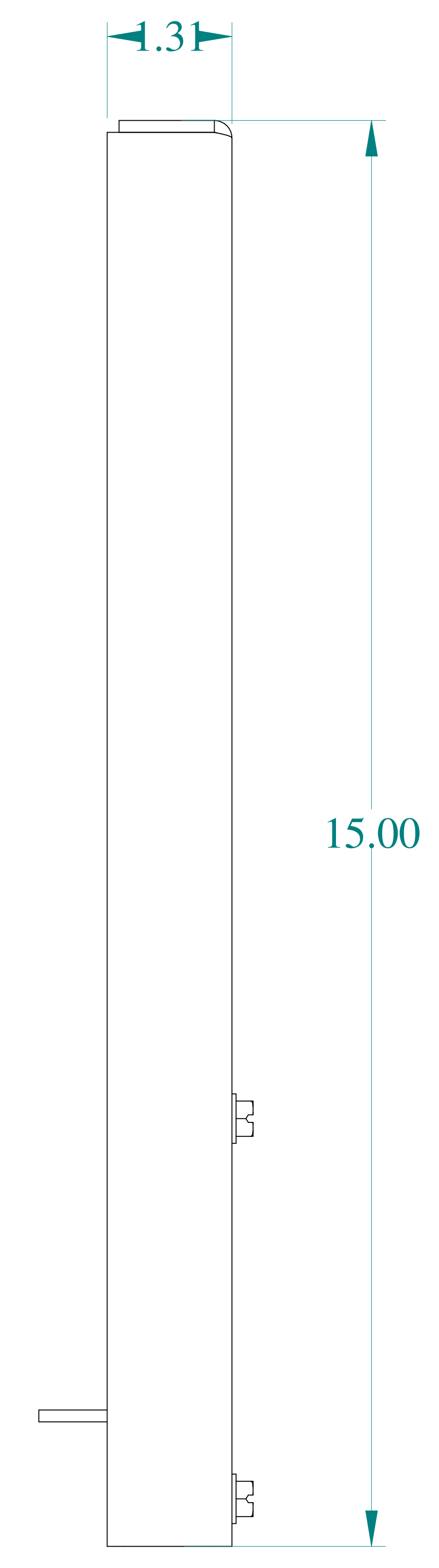
SIDE VIEW
