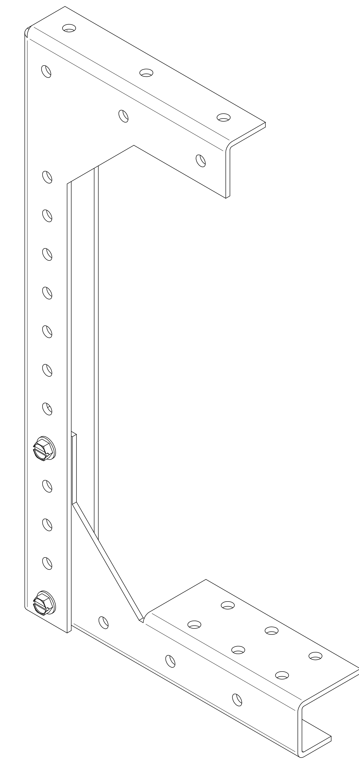
ISOMETRIC VIEWS
