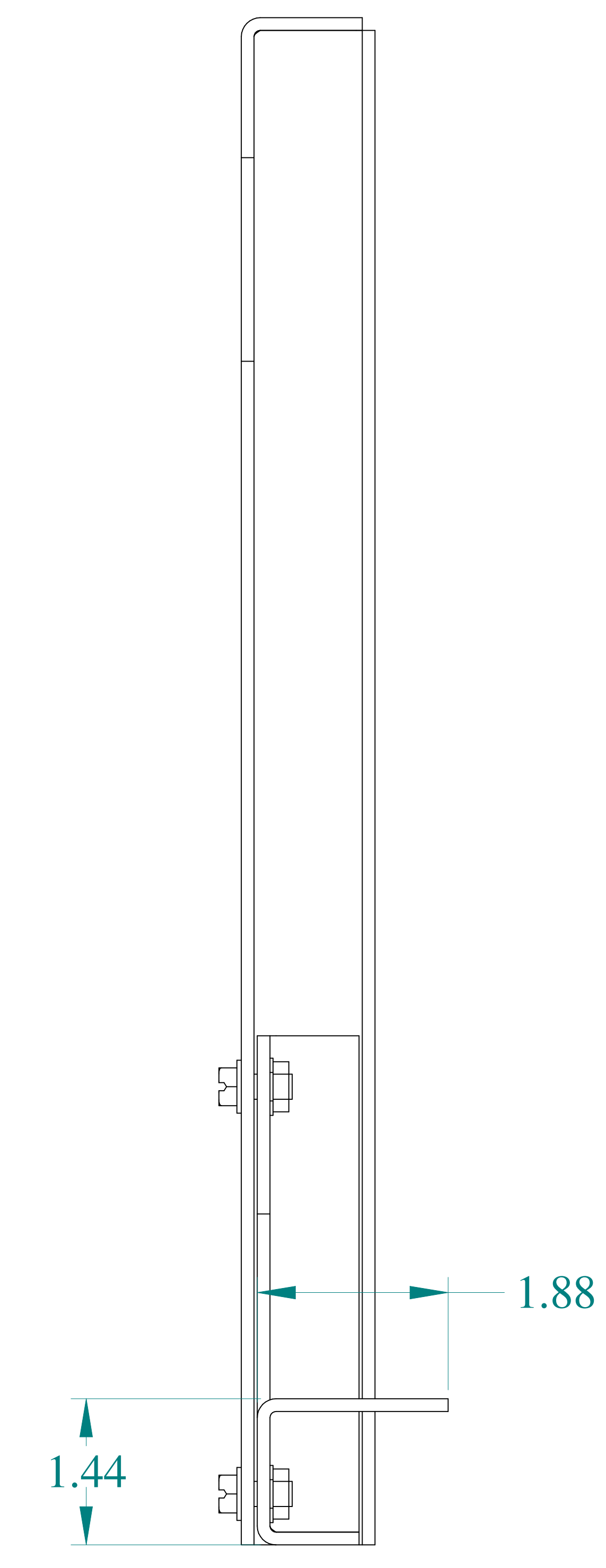
SIDE VIEW
