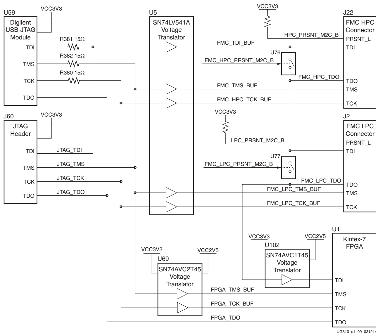
Figure 1-9: JTAG Circuit
