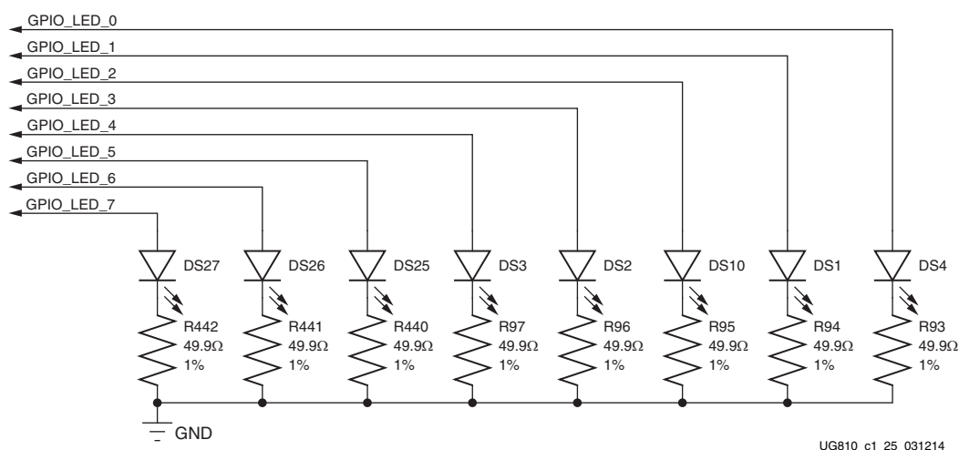
Figure 1-25: User LEDs
