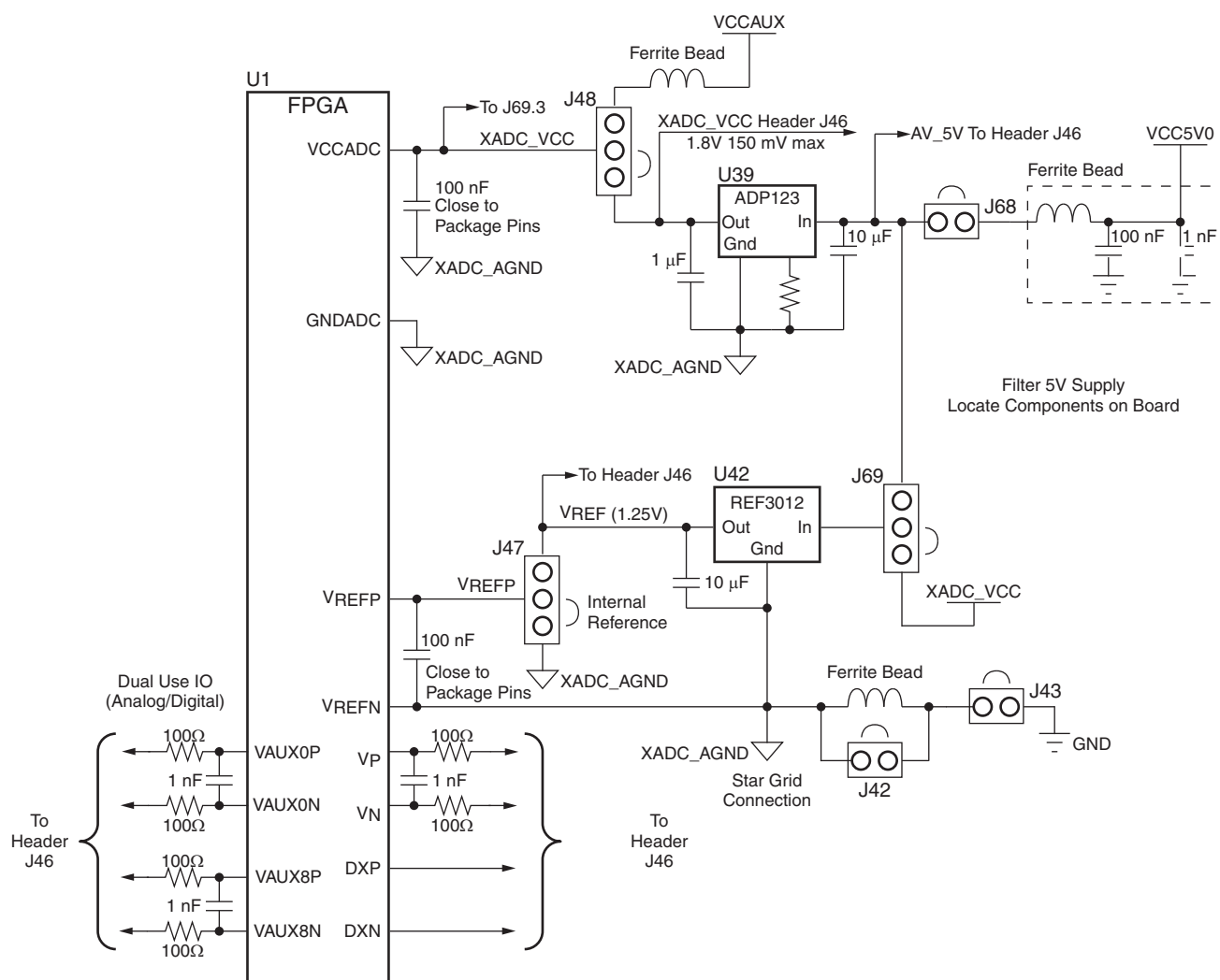
Figure 1-37: Header XADC_VREF Voltage Source Options
