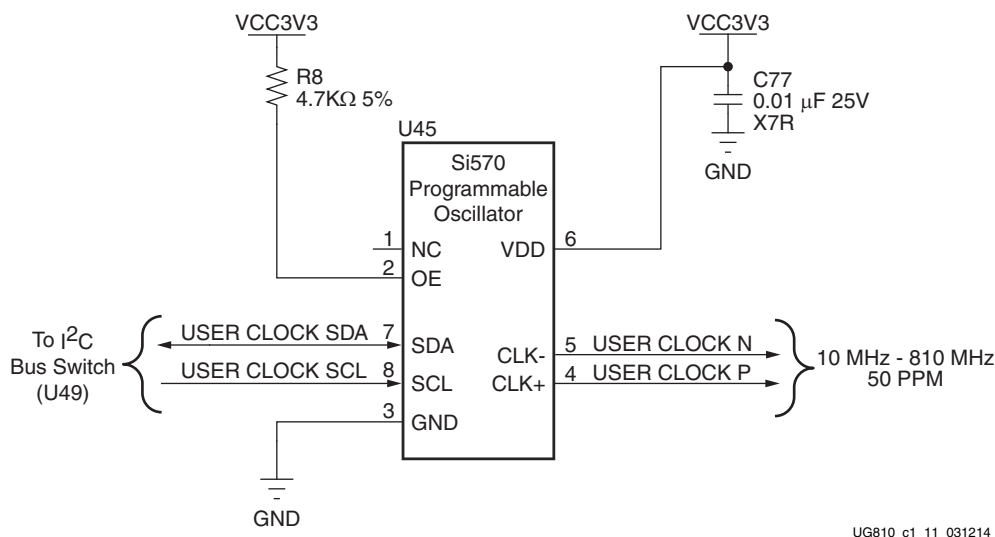
Figure 1-11: User Clock Source
