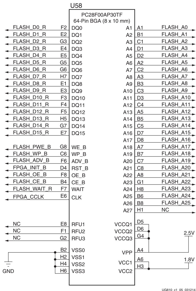
Figure 1-5: 128 MB Linear Flash Memory (U58)
