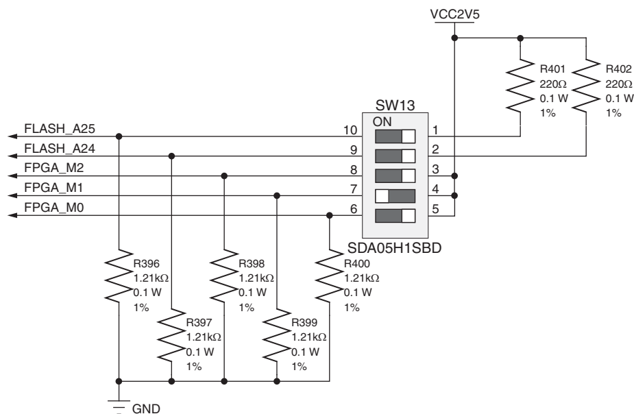
Figure 1-39: Mode Switch
