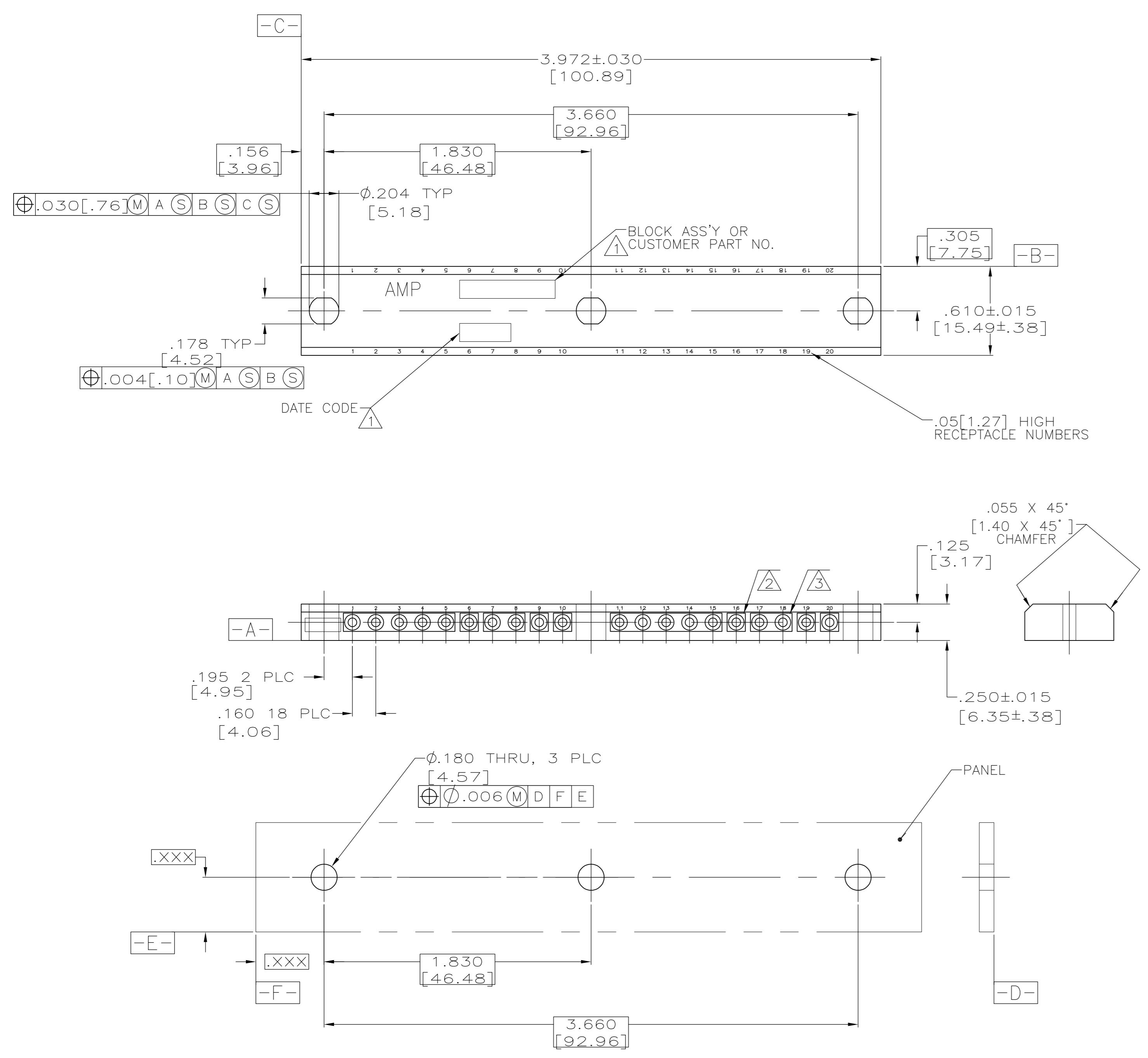
MOUNTING DIMENSIONS
