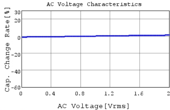
GRM188R71H331KA01 C-AC Voltage capchange, Dc
