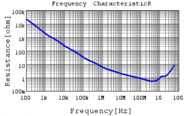
GRM188R71H331KA01 R DCOV,25degC
