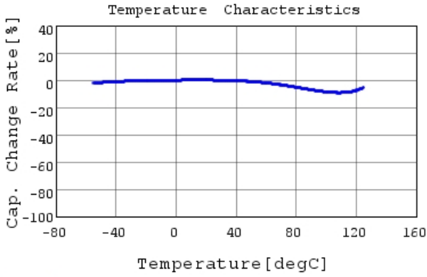
GRM188R71H331KA01 C-Temp. capchange, DC0.0V,
