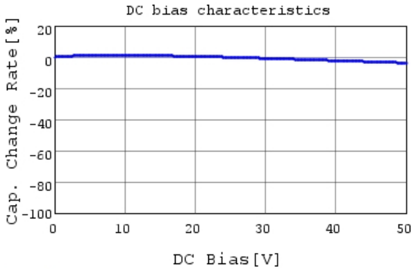
GRM188R71H331KA01 C-DC bias capchange, 25.0c
