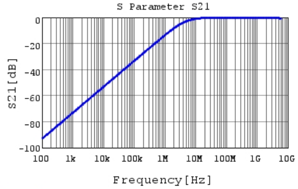
GRM188R71H331KA01 S21 DC0V, 25degC
