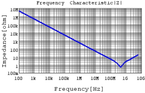
GRM188R71H331KA01 |Z| DCOV,25degC
