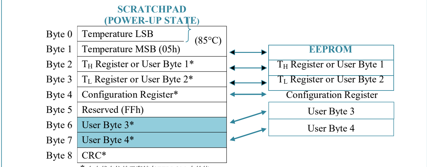
Figure7. GX18B20SH Memory
