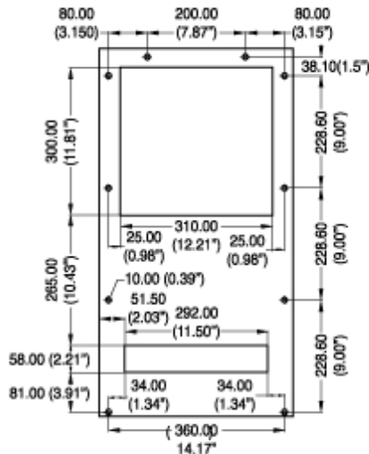
Drilling Template
