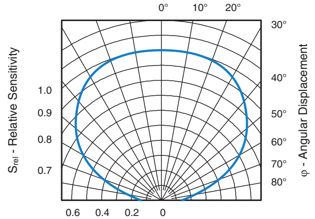
Fig. 6 - Relative Sensitivity vs. Angular Displacement
