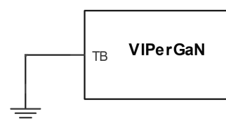
Figure 24. TB pin: external configuration (no dynamic blanking time nor valley synch)
