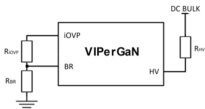
Figure 30. Brown-In/Out and input OVP: external configuration (Only BR)
