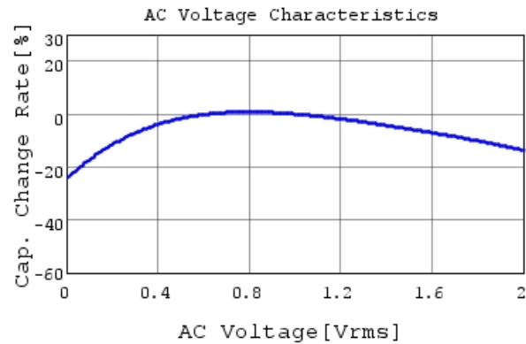
GRM033R61A105ME44 C-AC Voltage capchange, Dc
