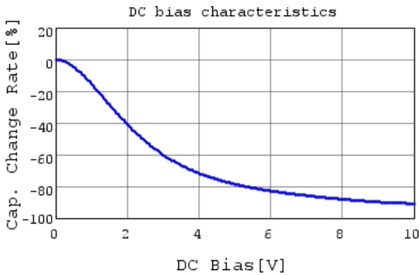
GRM033R61A105ME44 C-DC bias capchange, 25.0c
