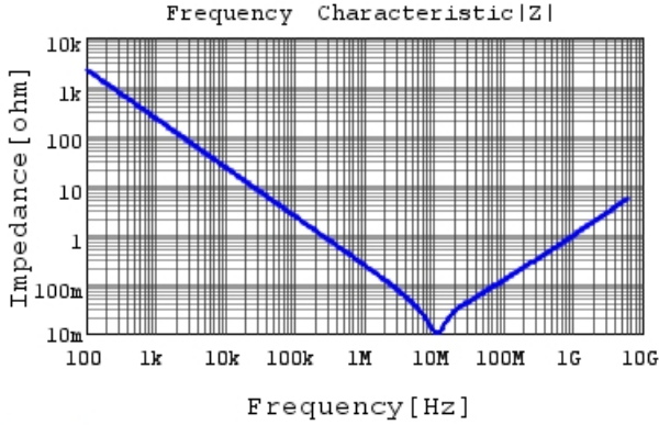
GRM033R61A105ME44 |Z| DCOV, 25degC
