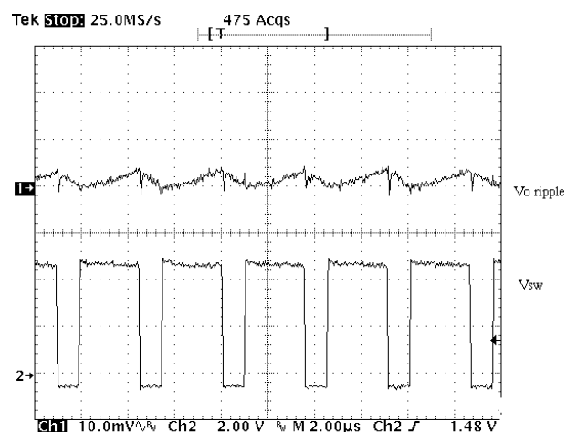
Figure 22. The Output Voltage Ripple Using One 100 \mu F POSCAP Capacitor
