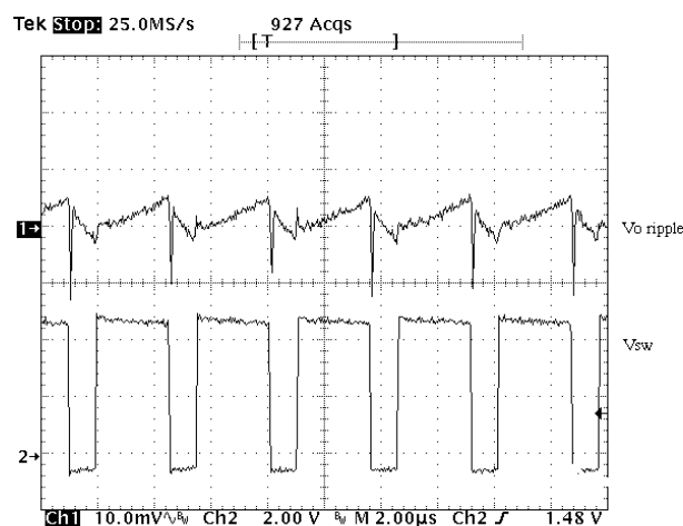
Figure 23. The Output Voltage Ripple Using One 100 \mu F OS-CON
