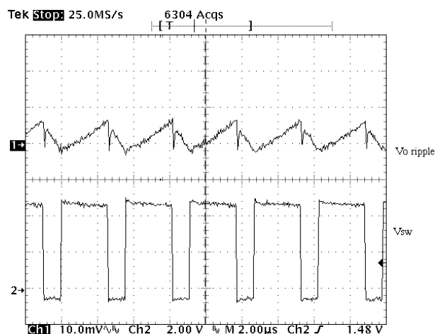
Figure 24. The Output Voltage Ripple Using One 100 \mu F Tantalum Capacitor
