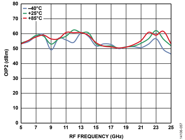
Figure 53. Output Second-Order Intercept (OIP2) vs. RF Frequency ( f_{RF} ) at a 7 dB Gain Setting for Various Temperatures, IF Amplitude = -15 dBm per Tone
