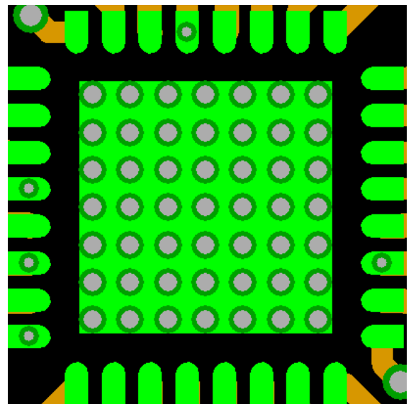
Figure 76. Evaluation Board Layout for the ADRF6780 Package
