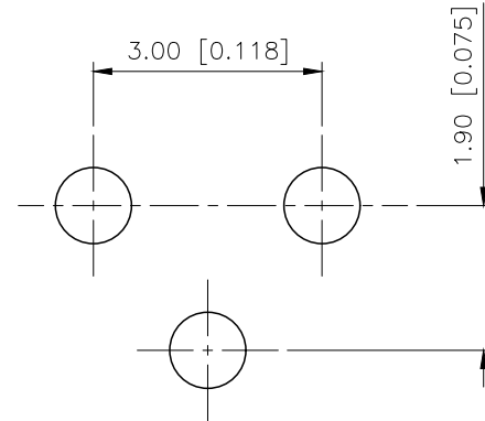
PCB Circuit prohibited area
