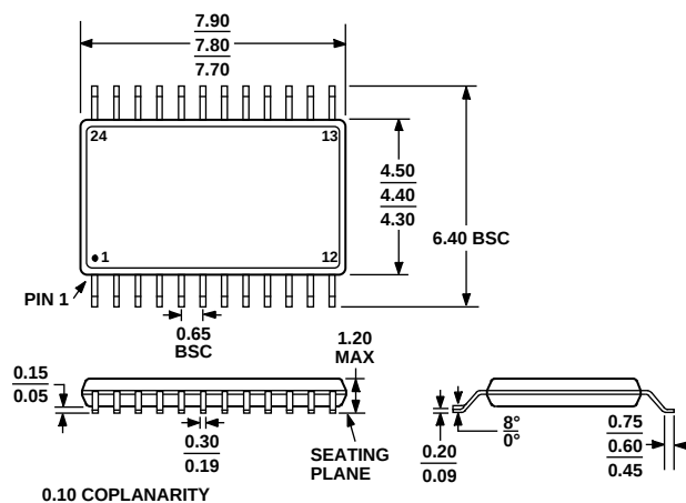
COMPLIANT TO JEDEC STANDARDS MO-153-AD Figure 51. 24-Lead Thin Shrink Small Outline Package [TSSOP] (RU-24)
