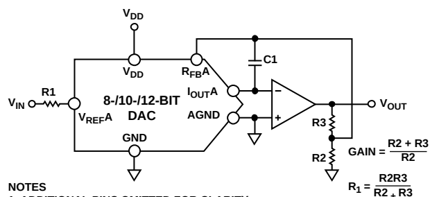
Figure 41. Increasing Gain of Current Output DAC
