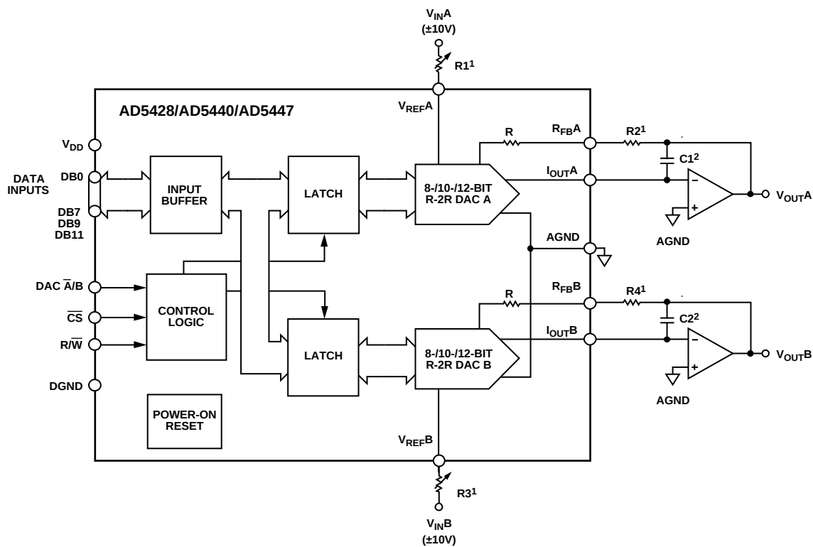
Figure 38. Unipolar Operation
