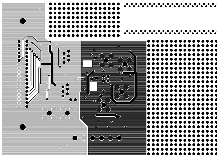
Figure 49. Solder-Side Artwork
