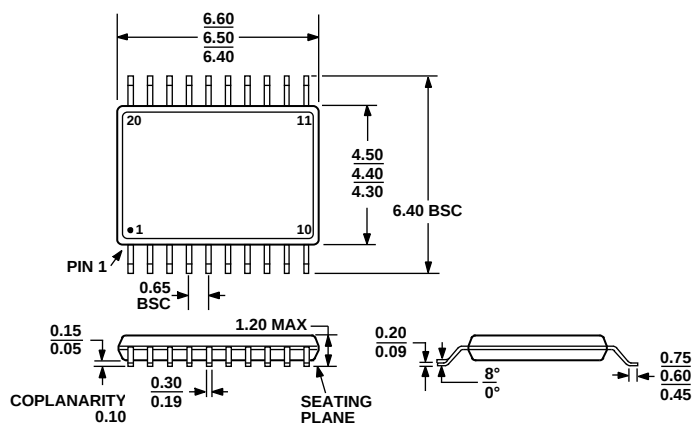
COMPLIANT TO JEDEC STANDARDS MO-153-AC Figure 50. 20-Lead Thin Shrink Outline Package [TSSOP] (RU-20)
