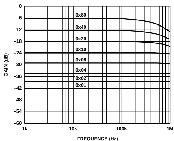
Figure 20. Gain vs. Frequency vs. Code, R_{AB} = 10\text{k}\Omega
