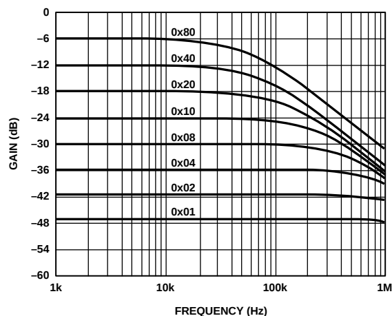
Figure 22. Gain vs. Frequency vs. Code, R_{AB} = 100\text{k}\Omega
