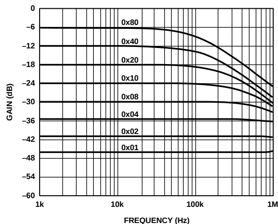
Figure 21. Gain vs. Frequency vs. Code, R_{AB} = 50\text{k}\Omega
