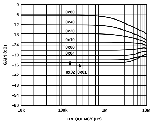
Figure 19. Gain vs. Frequency vs. Code, R_{AB} = 2.5\text{k}\Omega
