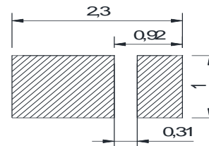
推荐焊盘尺寸 Recommended Soldering Pad
