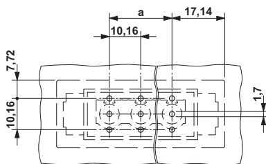
Drilling diagram
