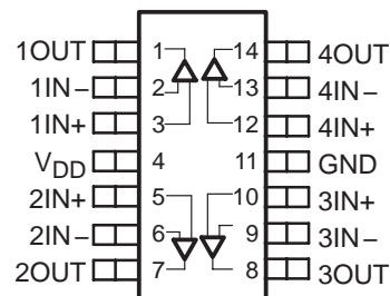
TLV2634 TSSOP-14/SOP-14
