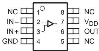
TLV2631 SOP-8
