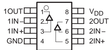
TLV2632 SOP-8
