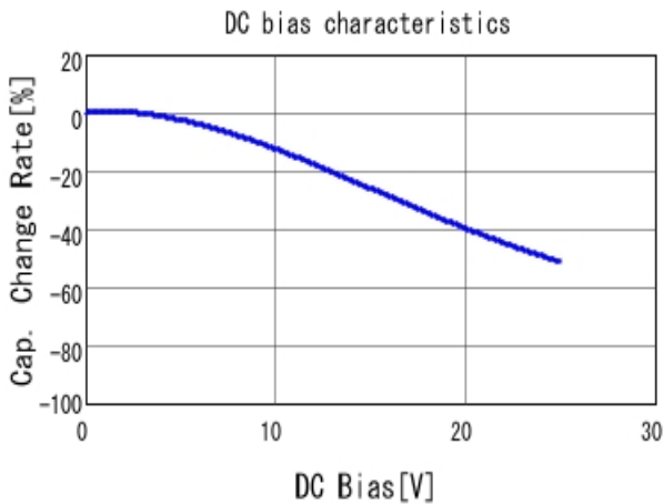
GCM21BR71E105KA56 C-DC bias capchange, 25.0degC, AC1.
