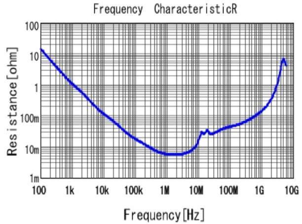
GCM21BR71E105KA56 R DCOV, 25degC
