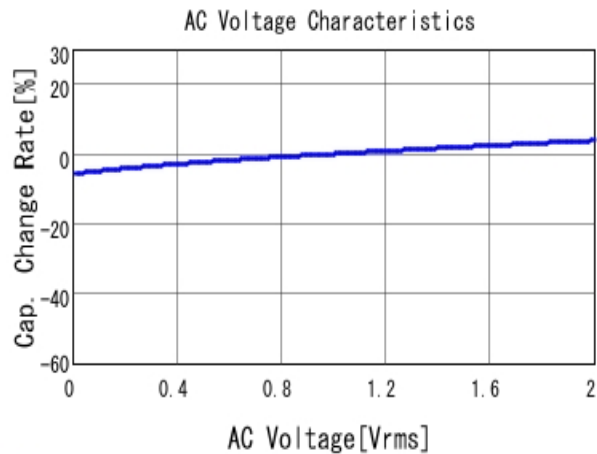
GCM21BR71E105KA56 C-AC Voltage capchange, DCOV, 25.0d
