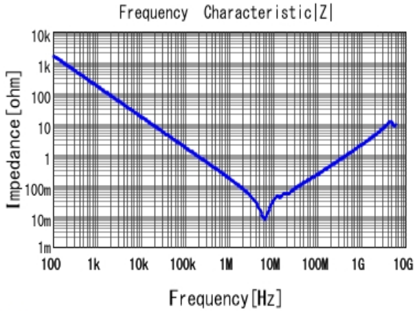
GCM21BR71E105KA56 |Z| DCOV, 25degC
