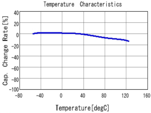
■ GCM21BR71E105KA56 C-Temp. capchange, DC0.0V, AC1.0V r m
