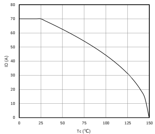
Maximum Drain Current I_D=f(T_c)
