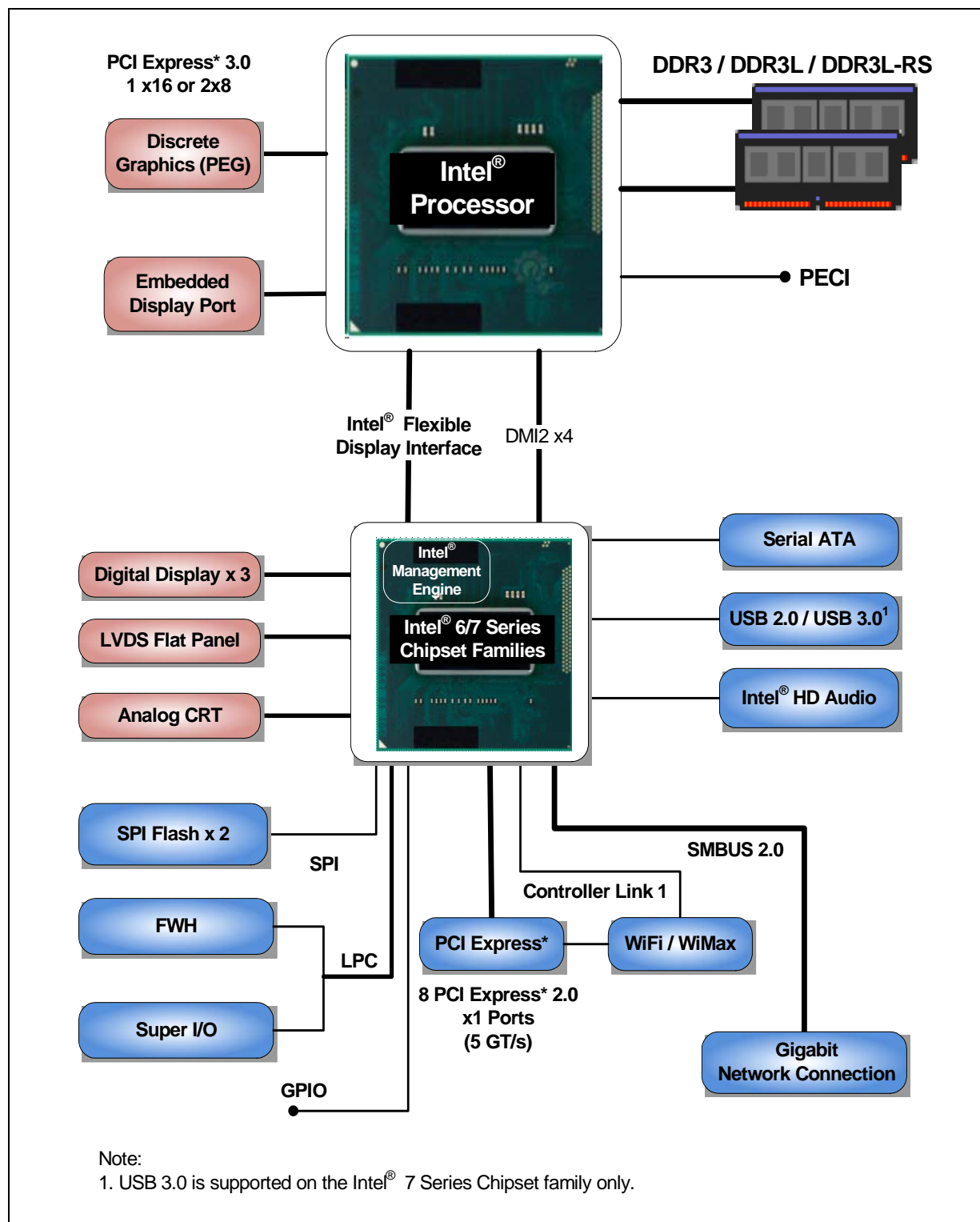
Figure 1-1. Mobile Processor Platform
