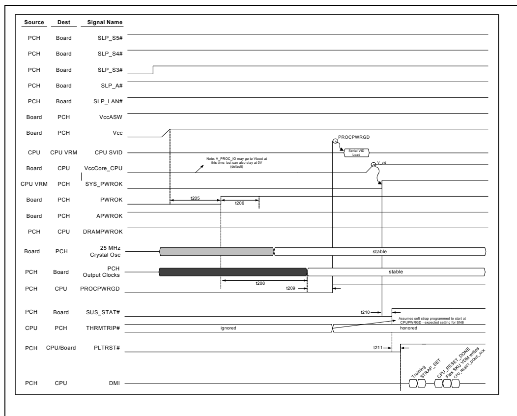
Figure 8-4. S3/M3 to S0 Timing Diagram
