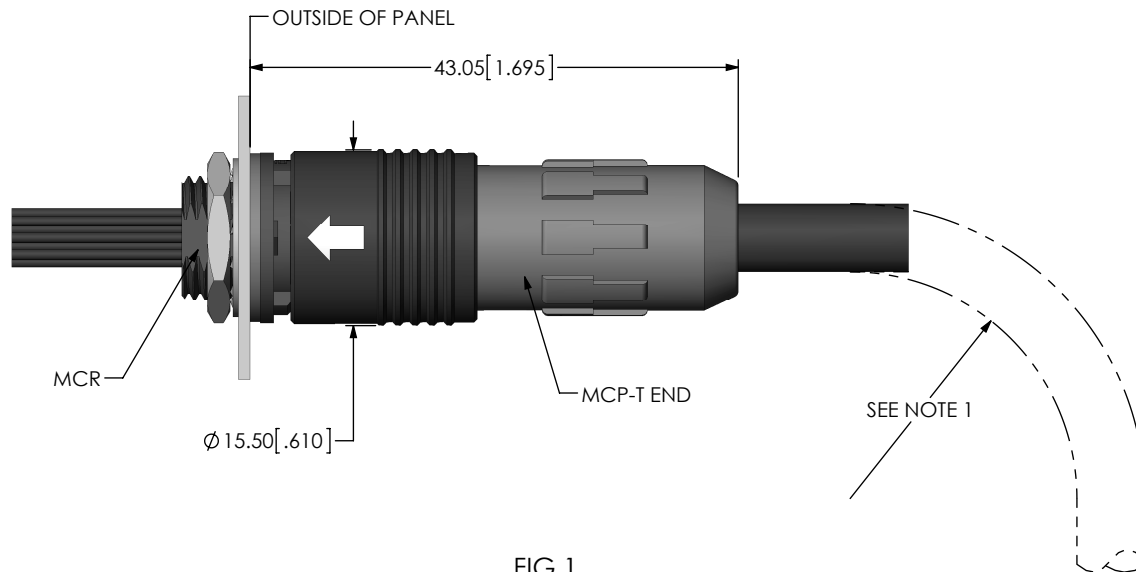
FIG 1 PANEL MATED VIEW
