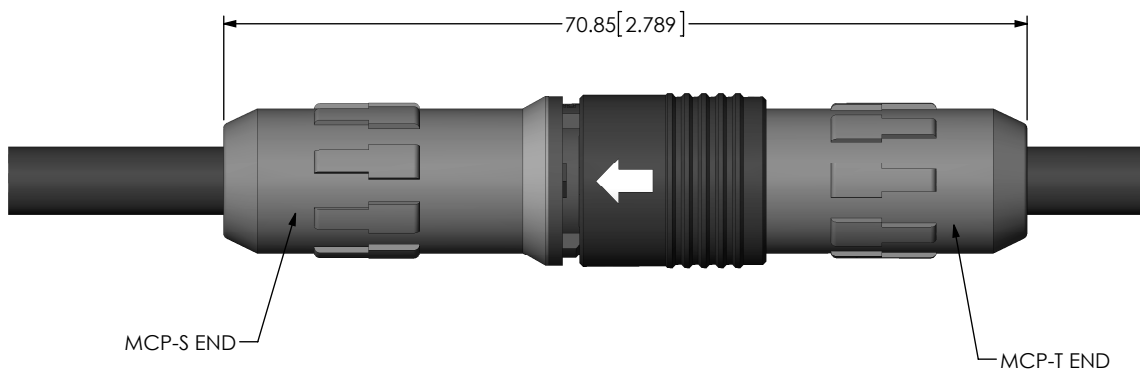
FIG 2 INLINE MATED VIEW
