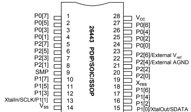
Figure 4: 26443 PDIP/SSOP
