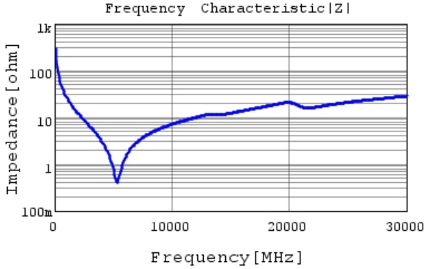
GRM0225C1H5R6CA03 |Z| DCOV, 25degC
