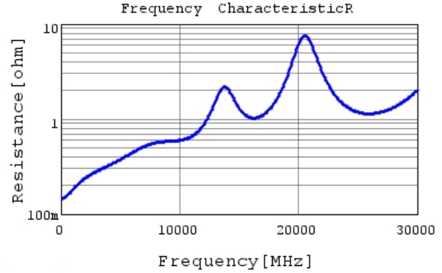
GRM0225C1H5R6CA03 R DCOV, 25degC
