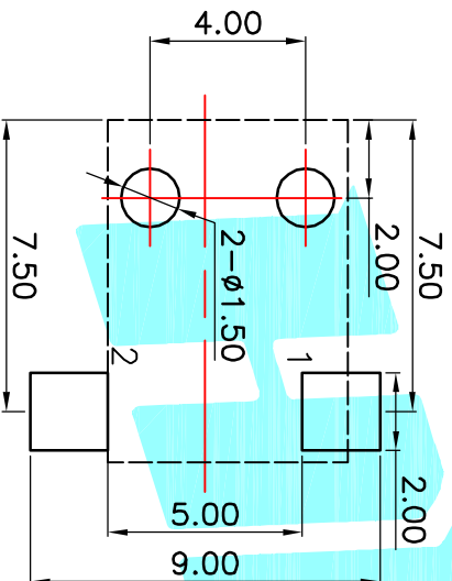
P.C.B LAYOUT(copper—sided view)
