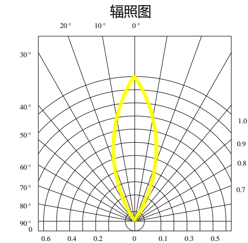
Radiation Diagram
