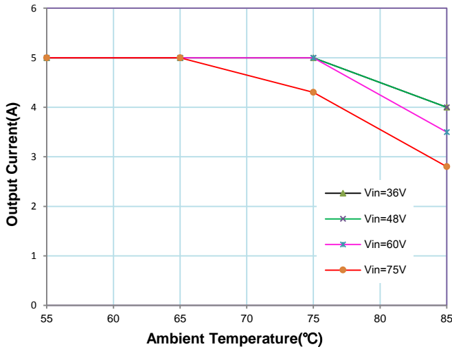
Power Derating
