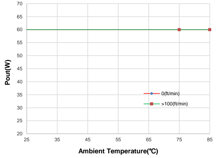
Power Derating (VIN=48V)
