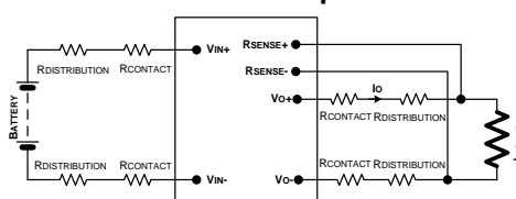
Fig 2. Output Voltage and Efficiency Test Setup
