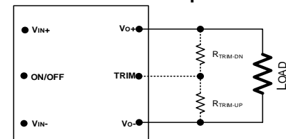
Fig 3. Output Ripple and Noise Test Setup
