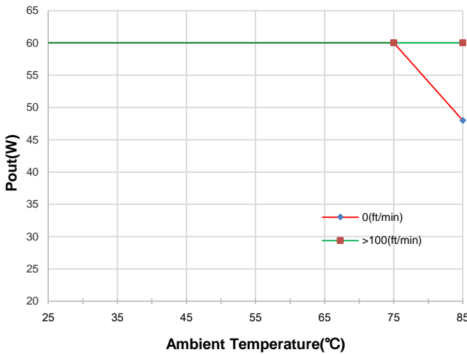
Power Derating (VIN=48V)
