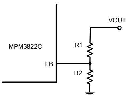
Figure 2: Feedback Network
