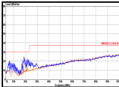
Radiated Emission
