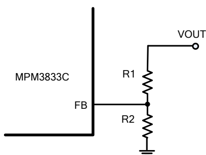
Figure 2: Feedback Network
