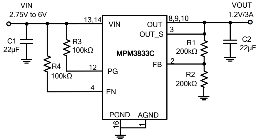
Figure 4: Typical Application Circuits for MPM3833C
