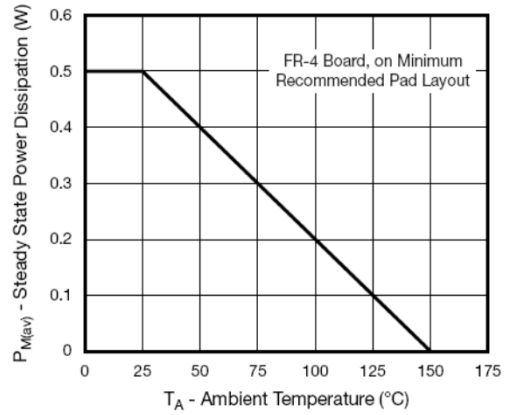
Fig. 2-Power Derating Curve
