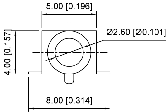
T:1.6 Dimensions of PC board holes Tolerance :±0.1(Printed-sided view)
