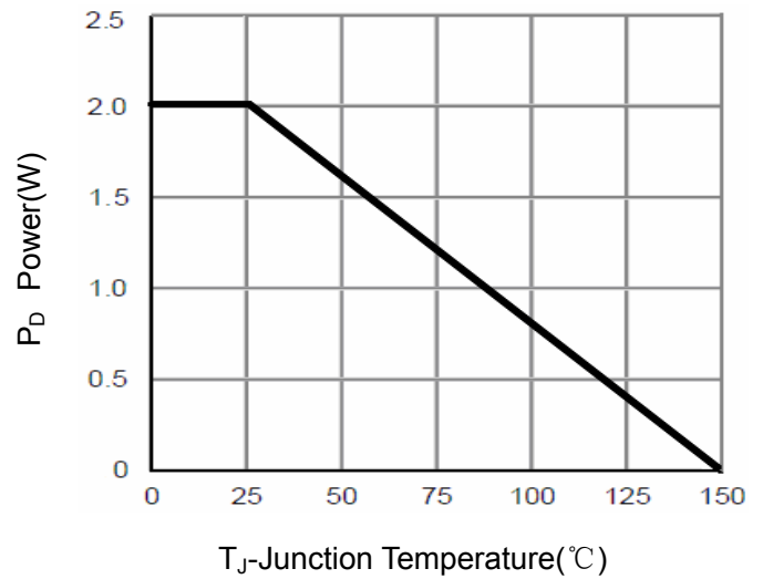
Figure 9 Power Dissipation
